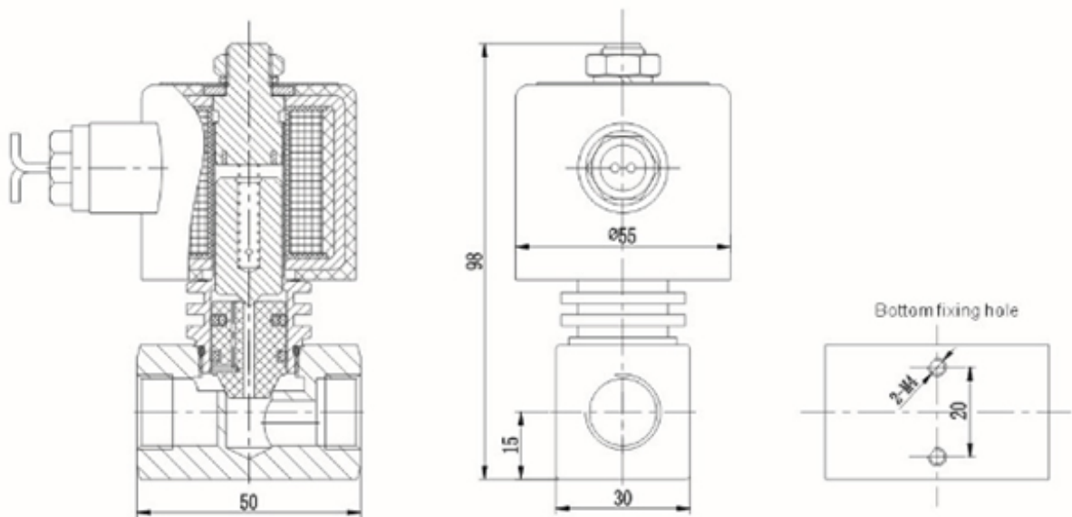
RSPS-08/10 steam solenoid valve drawing ( orifice size:φ8mm φ10mm thread:1/4 " 3/8 " )
