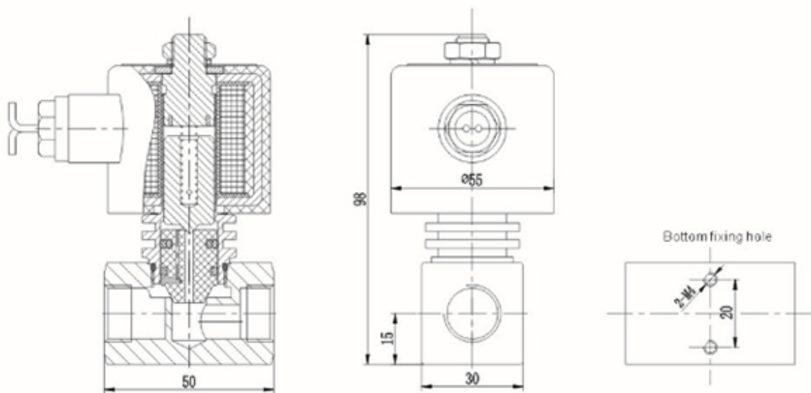
RSPS-08/10 steam solenoid valve drawing ( orifice size:φ8mm φ10mm thread:1/4 " 3/8 " )
